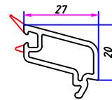
Glass Bead 6mm
