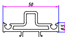
Inter-Seal for Sliding Sash 70&85mm
